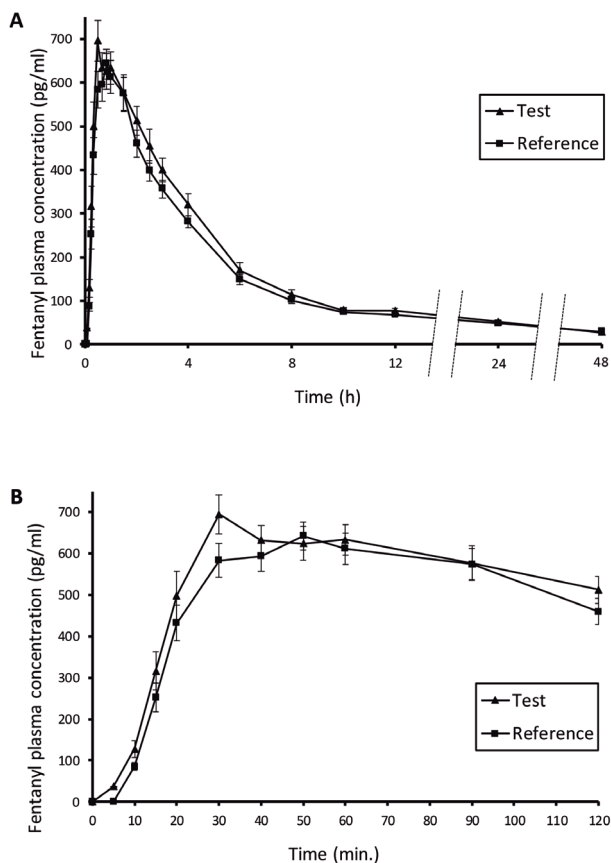
Fig. 1. Mean ± standard error of fentanyl plasma concentration versus time after single doses of 400 µg of Fentanyl Geiser Pharma (test) compared to 400 µg of Actiq (reference) in healthy adult volunteers (n = 36) for the first 48 h (A) and for the rapid absorption phase (B). At 72 h only 1 quantifiable sample was found (subject 05, test formulation, 23.7 pg/ml) and is not represented.
